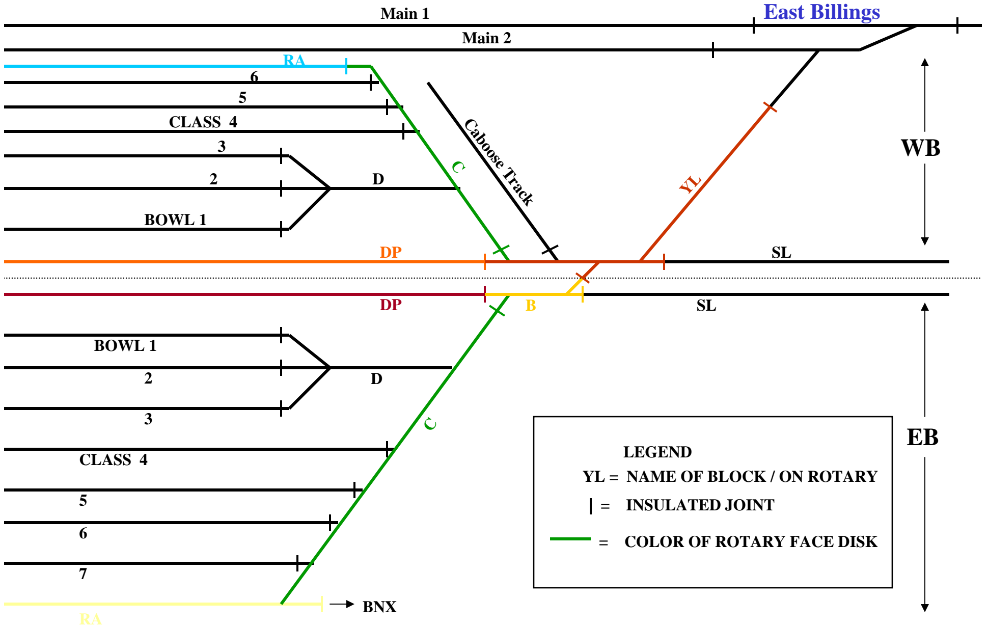
East end of Laurel Yard diagram.
